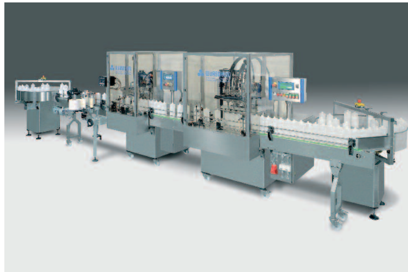
AFS 1000-4 / AV-200 Filling and capping line for liquid and pasty products.
